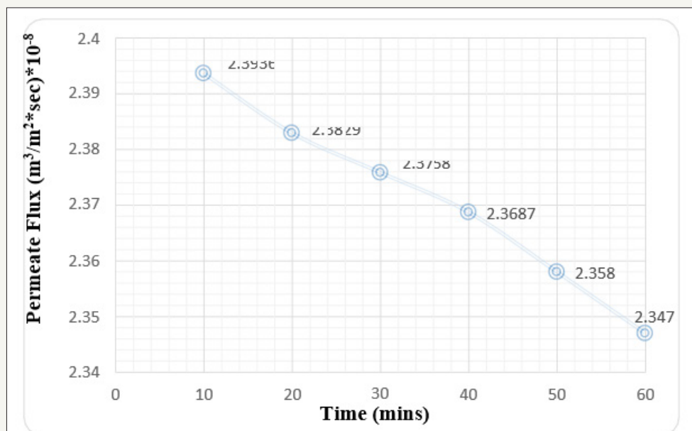
Figure 4: Graph of Permeate flux v/s time at 2 bar pressure keeping 1 ppm concentration (Before Cleaning).
